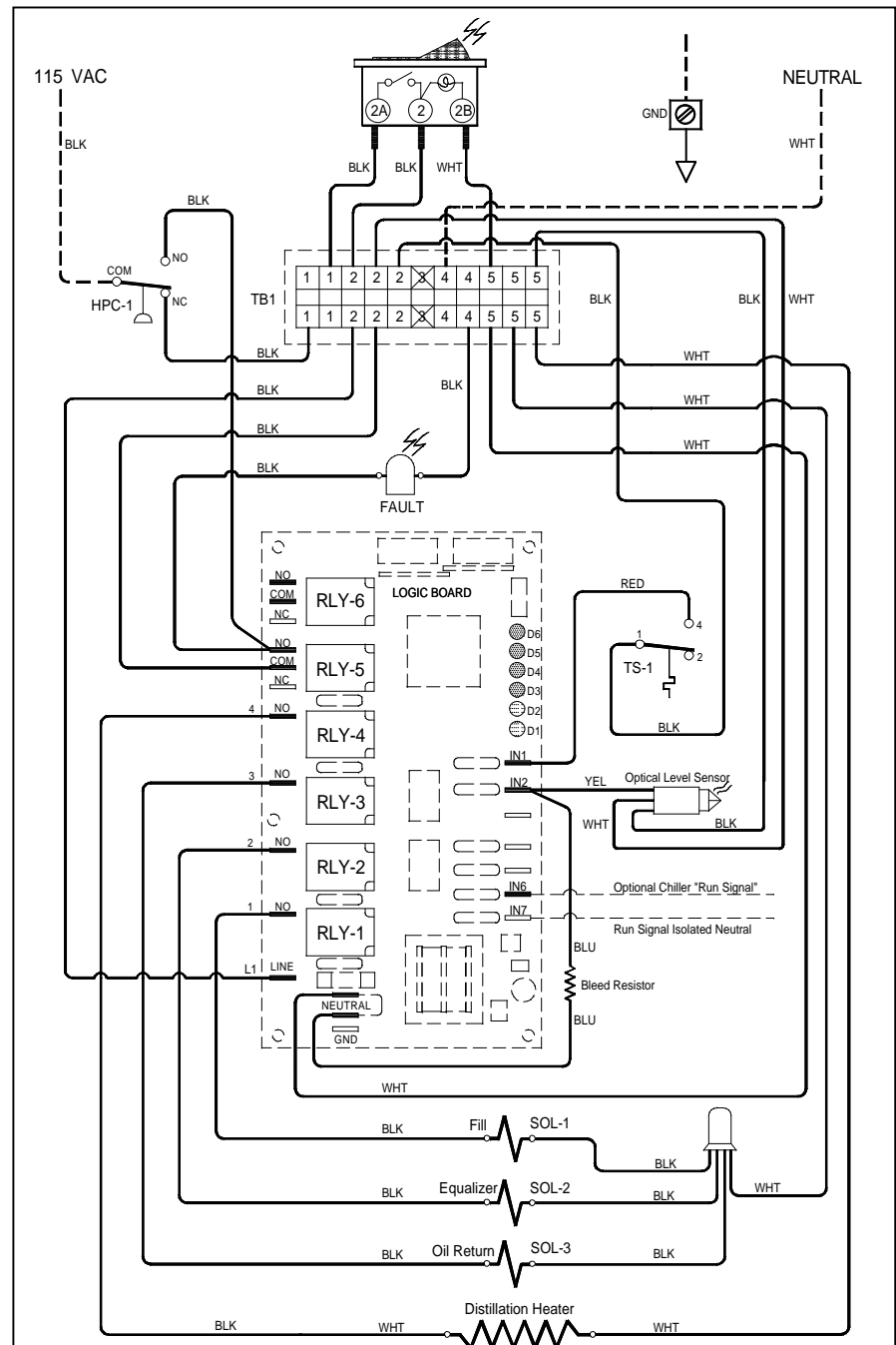
Wiring Schematic Model OAM-200
